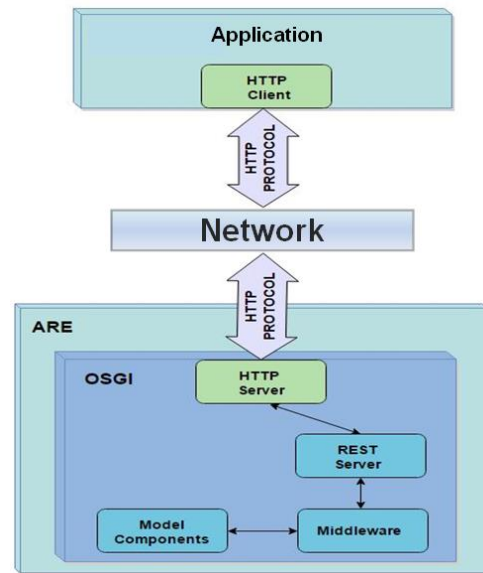
Figure 3. The REST-enabled AsTeRICS architecture.
